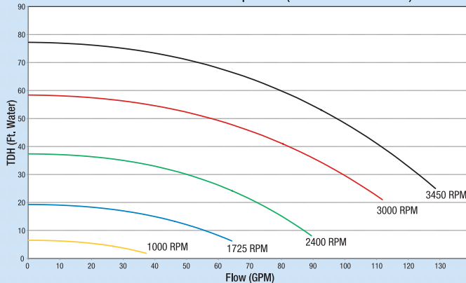
TriStar VS Performance Comparison (same for both models)
